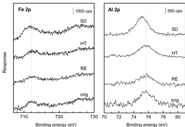
Fig. 5. XPS spectra of the Fe 2p and Al 2p peaks of Fe-BEA zeolites.
